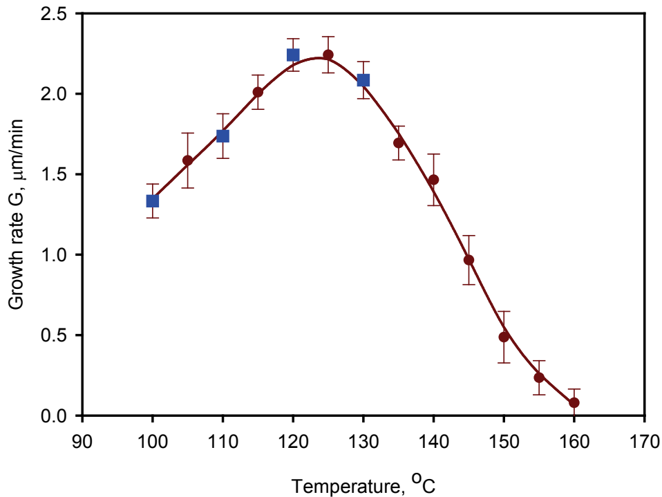
Figure 7.9. The experimental spherulitic growth rate of the poly(L/D-lactide) used in this study. Data are taken from Yuryev et al. [78]. The square symbols highlight the experimental conditions of this study.
