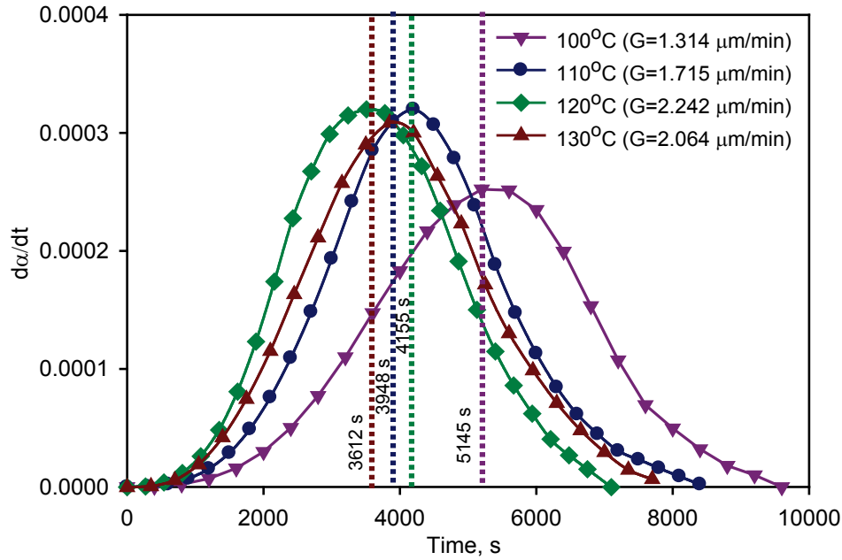
Figure 7.10. The simulation of bulk crystallization kinetics of the system having N=1 \times 10^8 \text{s}^{-1}\text{m}^{-3} with different growth rates. The dashed lines represent the half-time \tau_{1/2} of crystallization.
