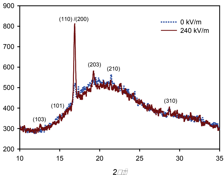
Figure 9.3. An overlap of the XRD profiles of the polylactide samples subjected to crystallization for 9000 s at 147.5 °C without applied electric field (dotted blue line) and under the influence of 240 kV/m electric field (solid red line).
