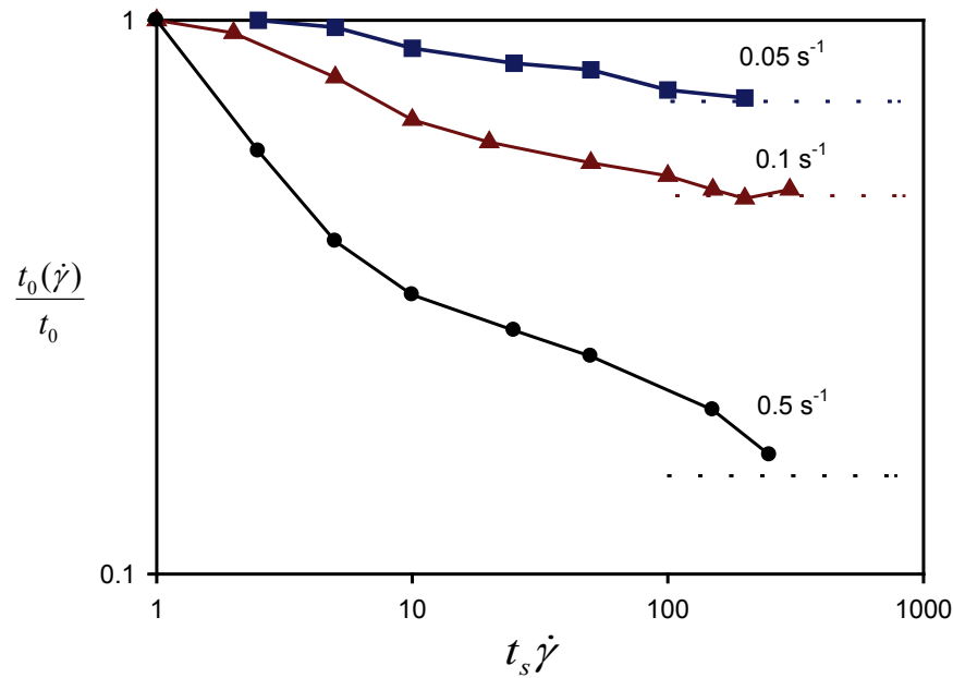
Figure 10.6. The relative induction time after the application of step shear. The temperature was 145^\circ\text{C} . The X axis represents the product of the shearing time and the shear rate. The dashed lines represent a reduced induction time for continuous shear.
