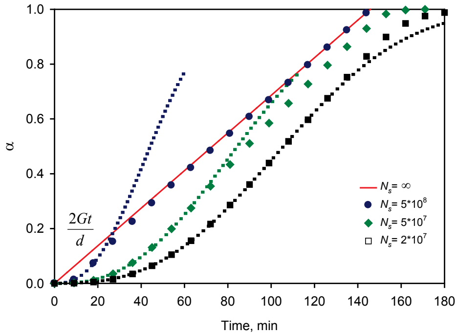
Figure 7.4. Kinetics of surface crystallization for different surface nucleation concentration. Data points are the simulation results for d=500 \mu\text{m} and G=1.715 \mu\text{m/min} . Dotted lines are fits of simulated crystallization data for the first stage of crystallization using Equation (7.7).
